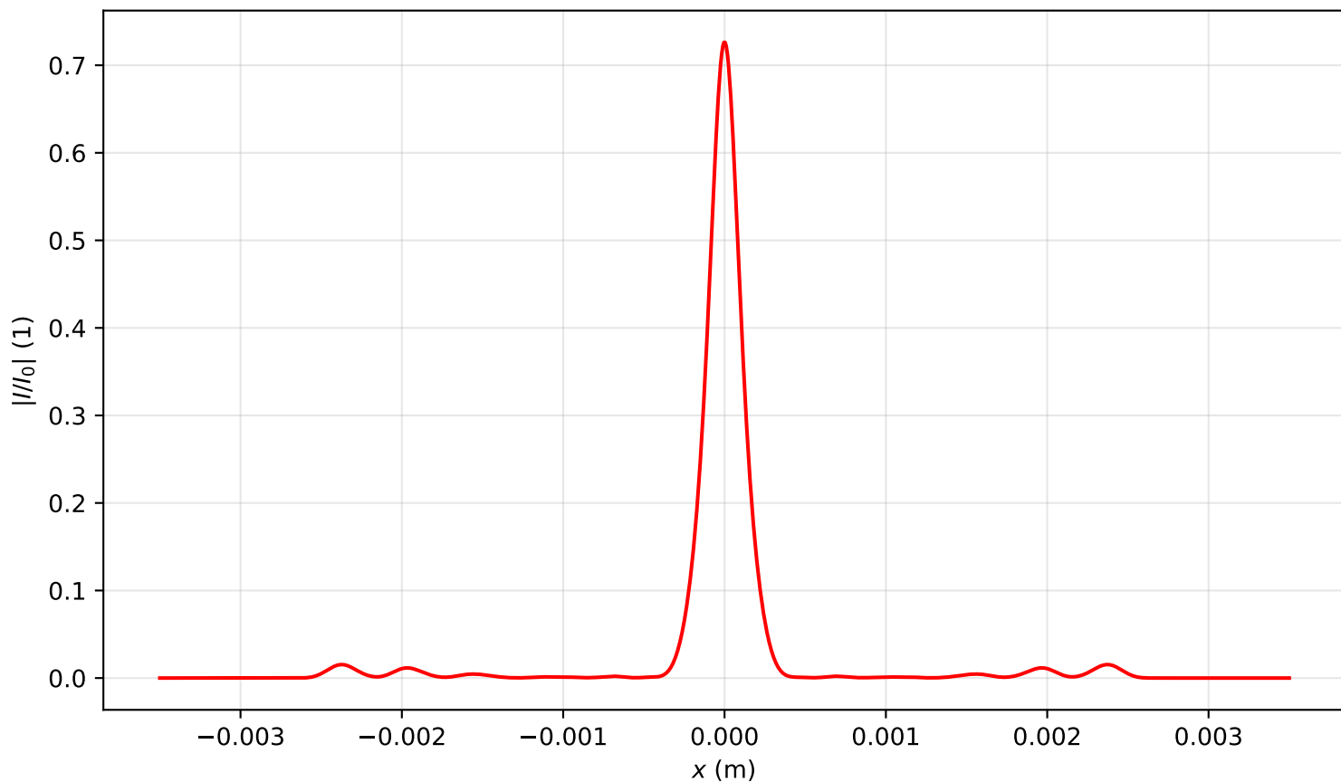
Intensity profile I(x, y = 0, z = 2.707)/I_0 , P_{in}=9.0P_{cr} , artificial time
